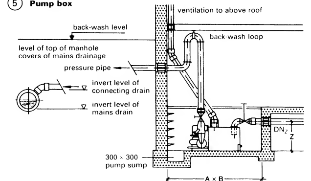
⑤ Pump box
